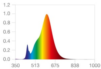
EPREL Data Spectral Diagram LEDr AC42296 2700K TW
