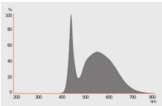
LISO spectral power distribution 6500K CRI90 v1
