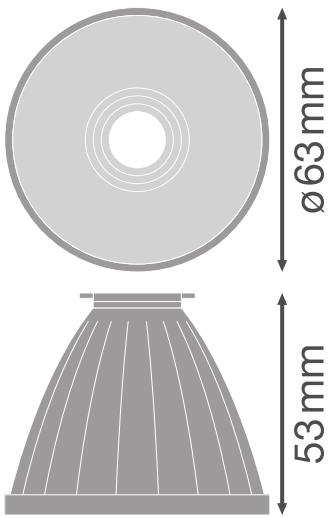
TRACK SP REFLECTOR D75
